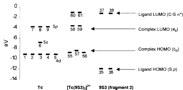
Fig. 5 Partial MO diagram for [Tc(9S3)] 2+ to show interaction between metal 4d-orbitals (FMOs 1–5; 3,4 and 5 have t 2g character) and ligand LUMO orbitals. For simplicity, ligand HOMO (FMOs 35, 36) and LUMO (FMOs 37, 38) orbitals from only one 9S3 (fragment 2) are shown.
